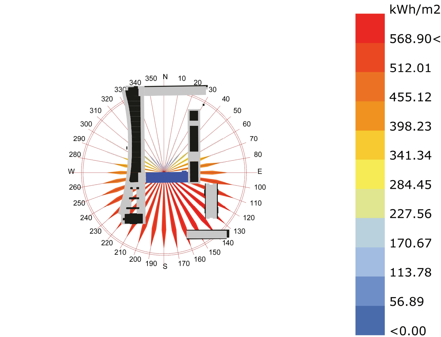
Direct Radiation(kWh/m2) London_ON_CAN_1975 1 JAN 1:00 - 31 DEC 24:00
